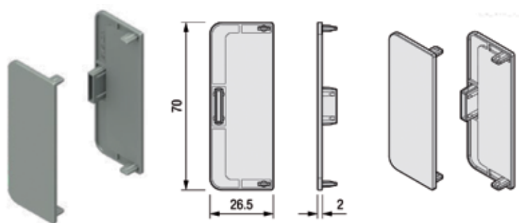
Embouts Gola C Led
