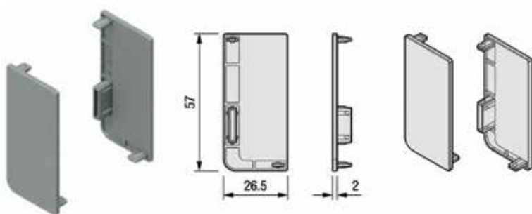
Embouts Gola L Led
